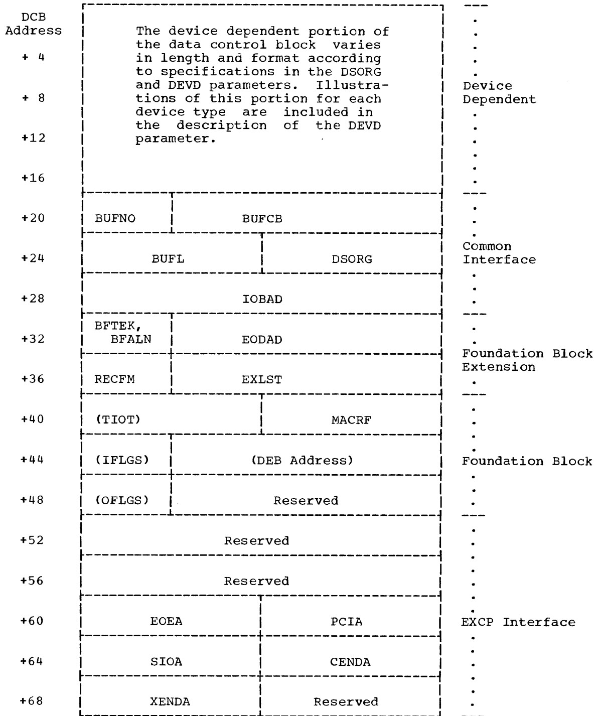
Figure 9. Data Control Block Format for EXCP (After OPEN)
