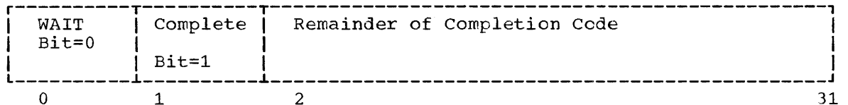
Figure 11. Event Control Block After Posting of Completion Code
