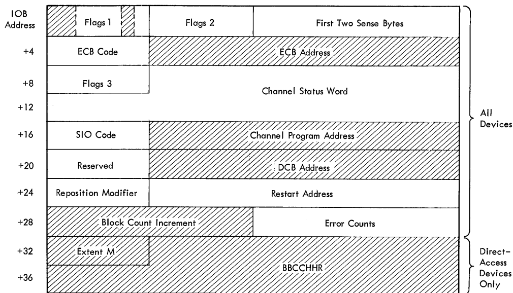
Figure 10. Input/Output Block Format
