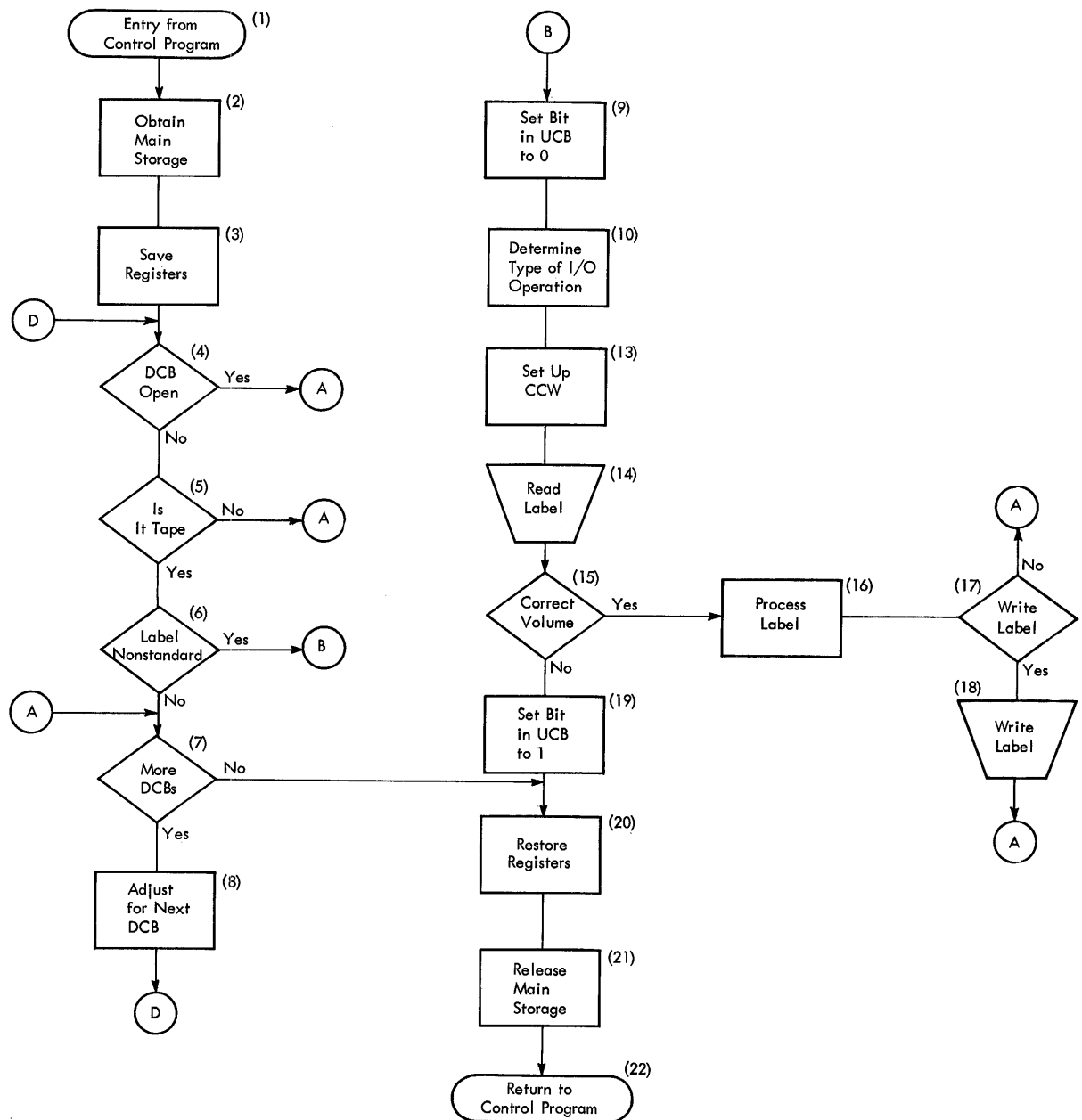
Figure 3. General Flow of a Nonstandard Label Processing Routine After Receiving Control From the OPEN Routine
